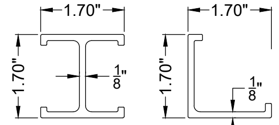
Line & End Post Aluminum Insert 6005A-T5
