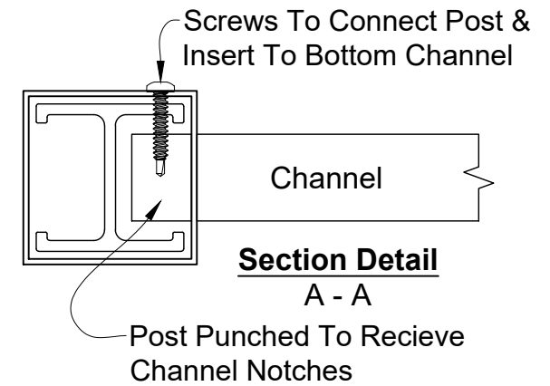
Line & End Post Aluminum Insert 6005A-T5
